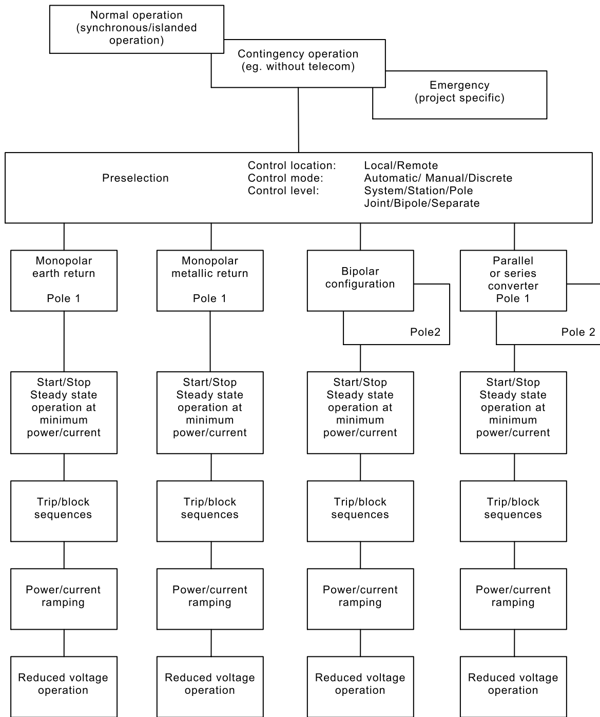
Figure 5 – Sequence for low power transmission tests
